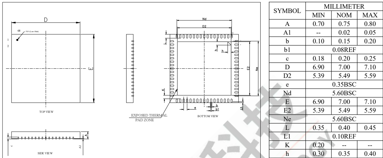
Figure 4-1 AC7925A Package
