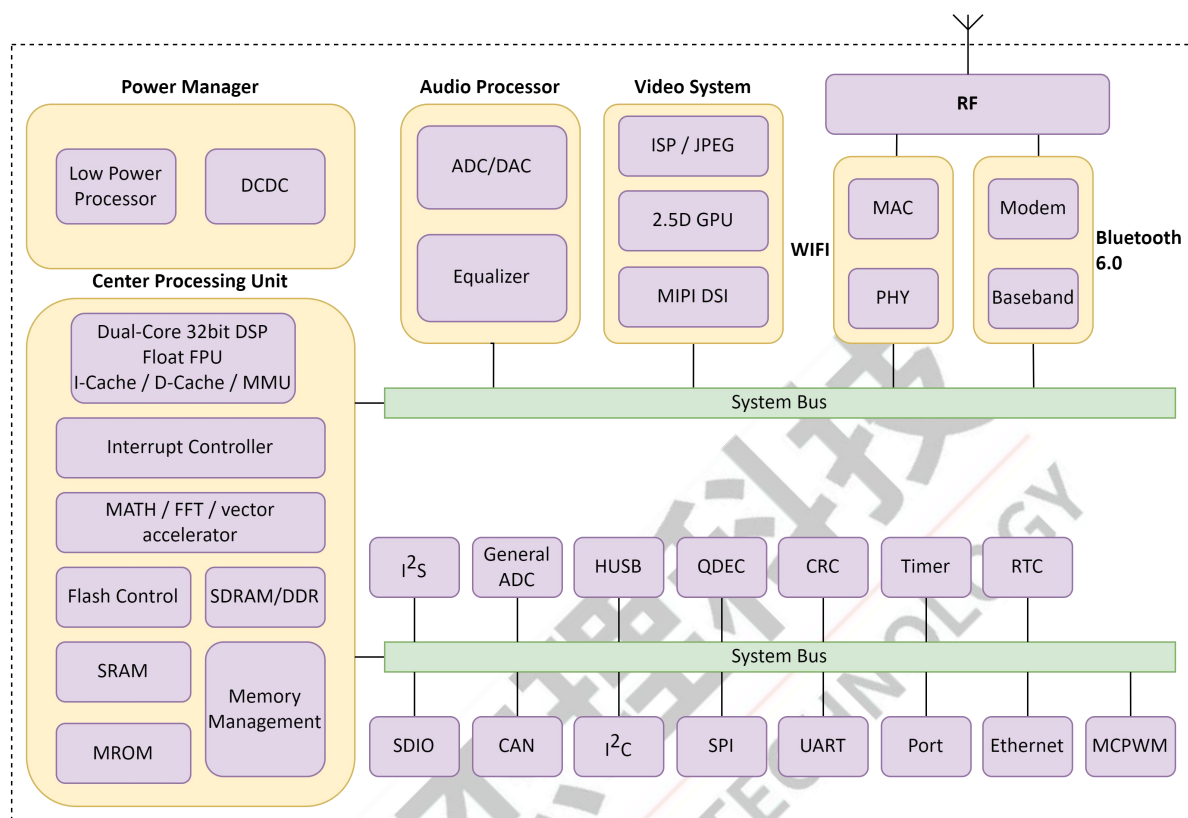
Figure 1-1 AC7925A Block Diagram
