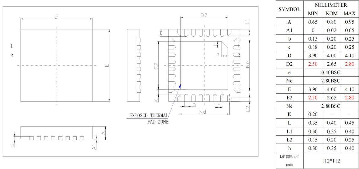
Figure 4-1 AC7106F Package
