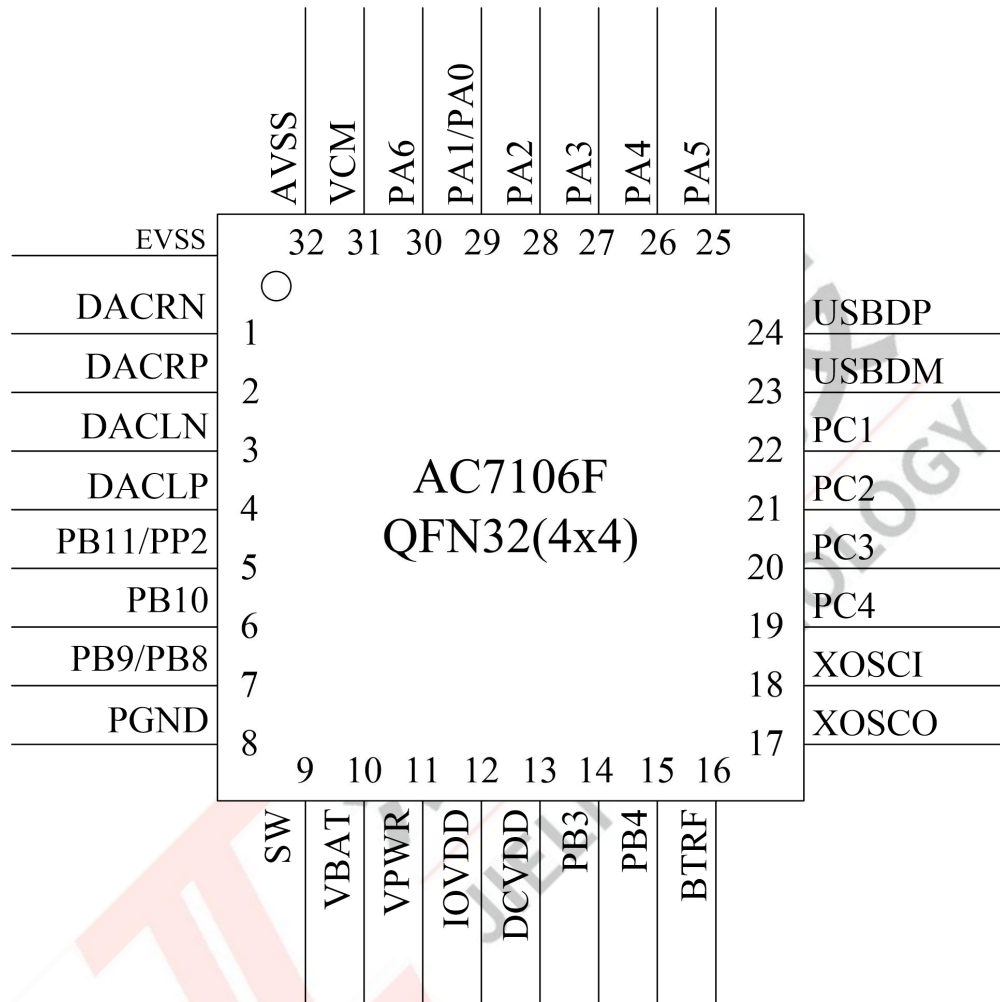
Figure 2-1 AC7106F Pin Assignment
