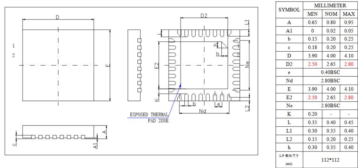
Figure 4-1 AC7106A Package
