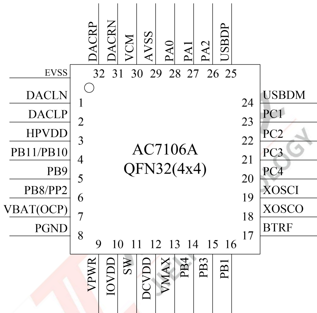
Figure 2-1 AC7106A Pin Assignment
