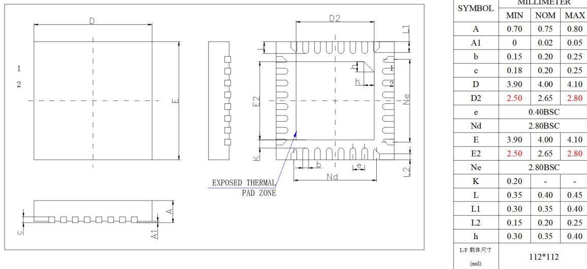
Figure 4-1 JL7096D Package
