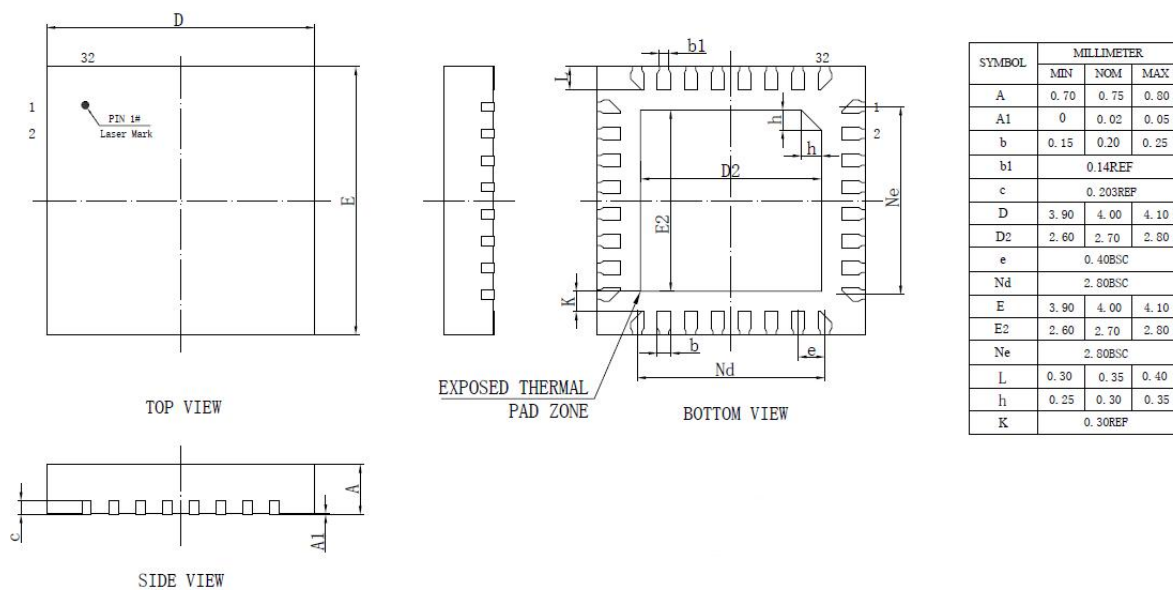
Figure 3-1 JL7006D Package
