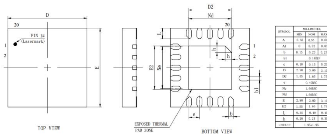
Figure 3-1 AC7003F Package
