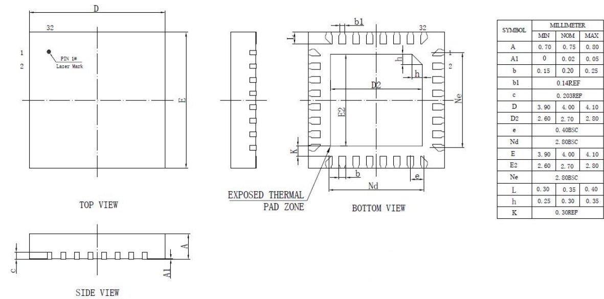
Figure 3-1 JL6976M Package
